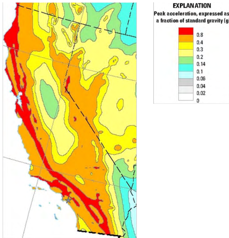
Figure 6-4: USGS 2014 Seismic Hazard Map - 2% Chance of Exceedance in 50 Years Peak Ground Acceleration (PGA) as a Percentage of Gravity (g)
